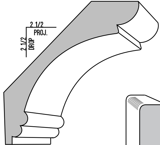
CROWN F611 - 3/4" X 3 5/8"
