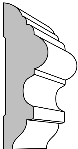
CHAIRRAIL F719 - 3/4" X 2 1/2"
