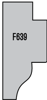
F639 - 3/4" X 1 5/8"
