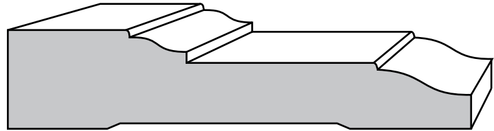
CASING F1442 - 3/4" X 3 1/2"
