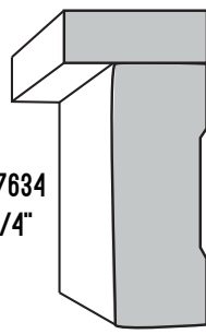
CHAIR RAIL CAP F1636 1/4" X 11/16"
