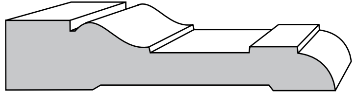
CASING F1422 - 3/4 X 3 1/2"
