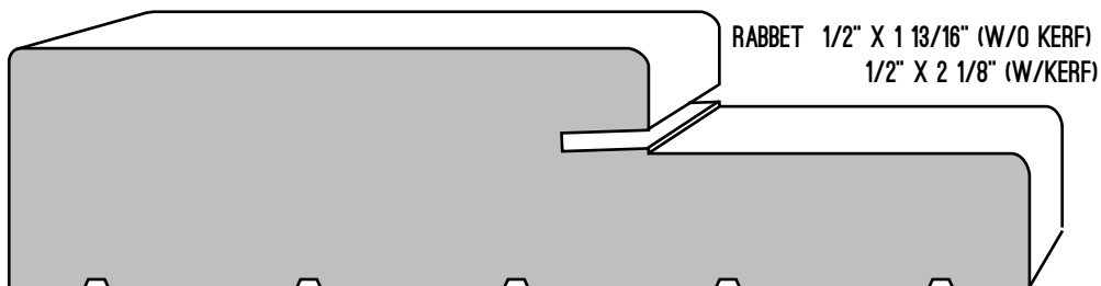
F365 A 1 3/16" X 4 9/16" F365E 1 3/16" X 4 13/16" F365K 1 3/16" X 5 3/8"
