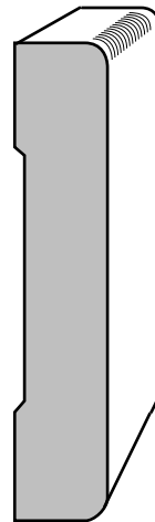
CHAIRRAIL F156 - 7/16" X 2 1/4"
