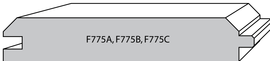
F775A - 3/4" X 3 1/4" F775B - 3/4" X 4 1/4" F775C - 3/4" X 5 1/4"
