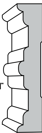
CHAIR RAIL F7654 7/16" X 2 1/4"
