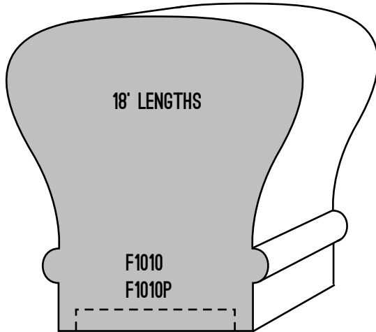
F1010 - 2 1/4" X 2 3/8" F1010P - PLOWED 3/16" X 1 1/4"
