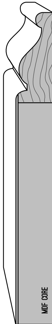
BASE F280 5/8" X 5 1/4"
