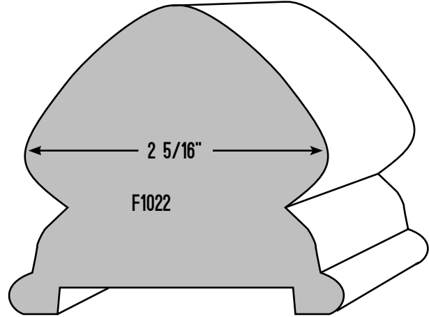
F1022 - 2 5/16" X 2 1/2" PLOW - 3/16" X 1 3/4"
