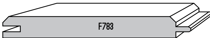
F783 - 3/8" X 3 1/4"
