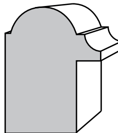
BACKBAND F1912 1" X 1 5/16"
