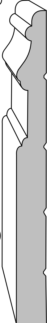
BASE F2410 - 1/2" X 5 1/4"
