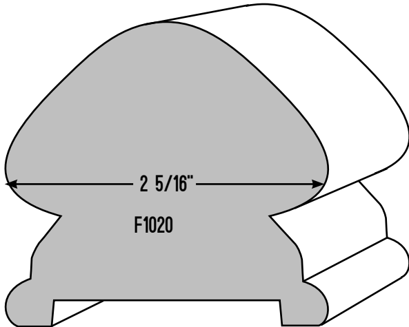
F1020 - 2 5/16" X 2 7/16" PLOW - 3/16" X 1 3/4"
