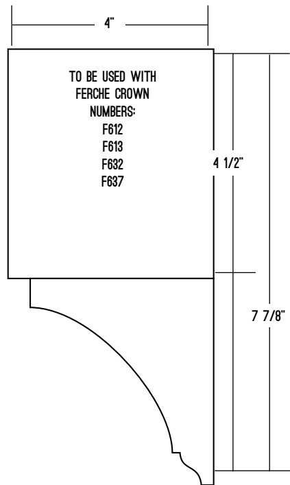
F645 - 4" X 4" X 4 1/2"
