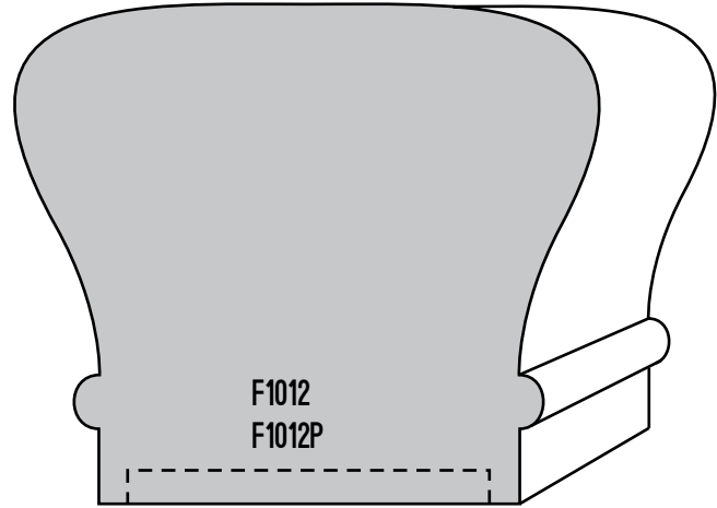
F1012 - 2 27/32" X 2 3/8" F1012P - PLOWED 3/16" X 1 3/4"
