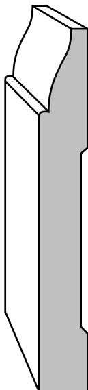
BASE F219 - 3/8" X 2 3/4"
