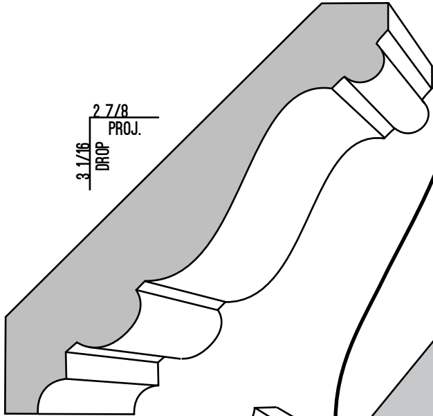
CROWN F6420 - 3/4" X 4 1/4"
