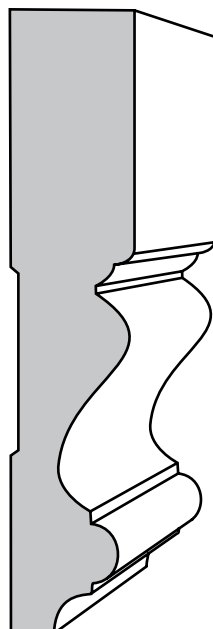
CROWN EXTENDER/APRON CASING F1413 - 5/8" X 3 1/4"
