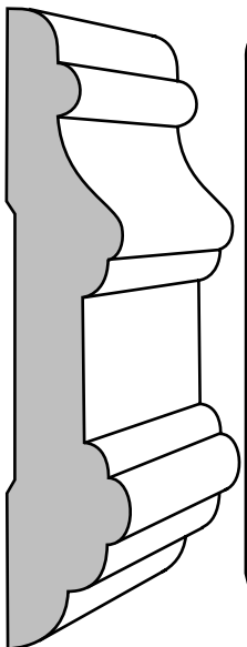
CHAIR RAIL F7410 9/16" X 3"
