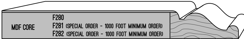
F280 - 5/8" X 5 1/4" F281 - 5/8" X 7 1/4" F282 - 5/8" X 9 1/4"
