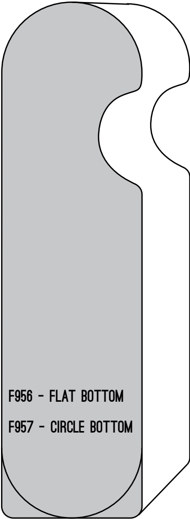
F956 - 1 1/2" X 5 1/2" F957 - 1 1/2" X 5 1/2"
