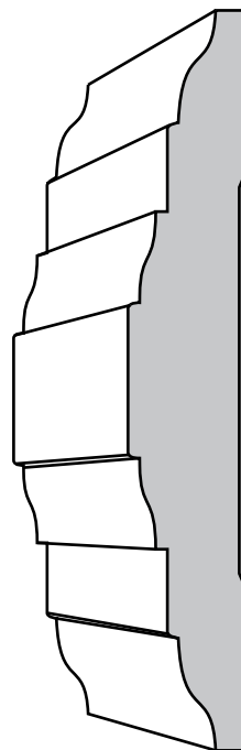
CHAIRRAIL F7442 - 9/16" X 3 1/2"
