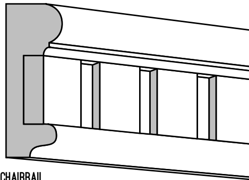
CHAIRRAIL F734 - 11/16" X 2 1/4" F735 (DENTIL) - 9/32" X 1"
