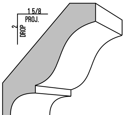
CROWN F615 - 9/16" X 2 5/8"
