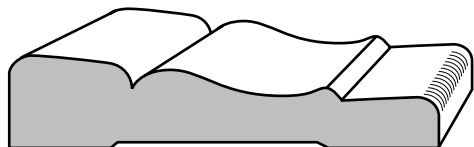
CASING F115 - 1/2" X 2 1/4"
