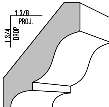
CROWN F608 - 9/16" X 2 1/4"
